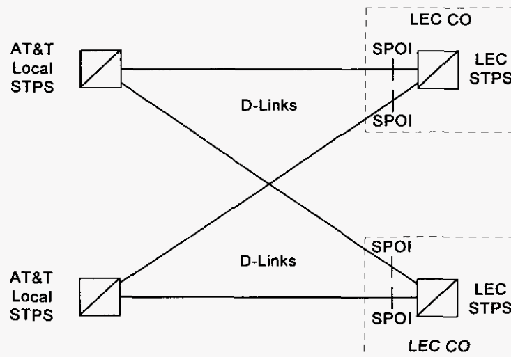
Figure 7. D-Link Interface
