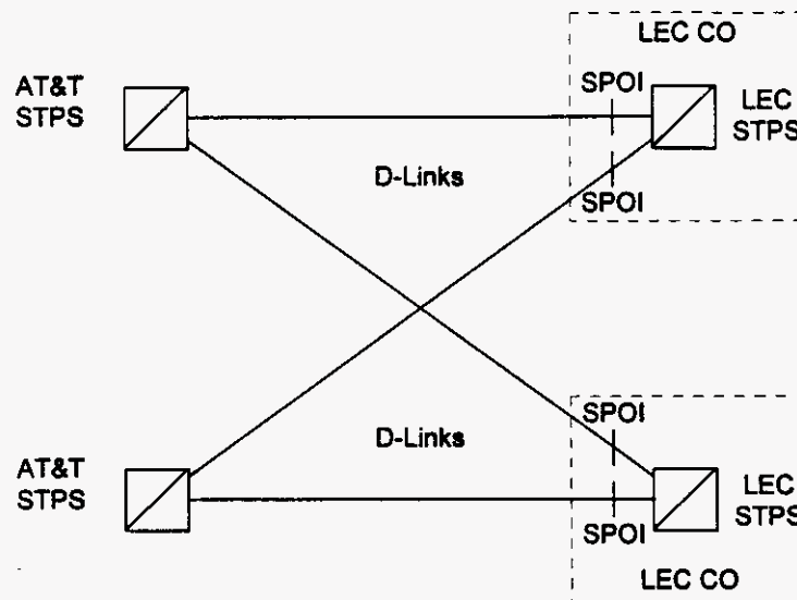
Figure 12. D-Link Interface
