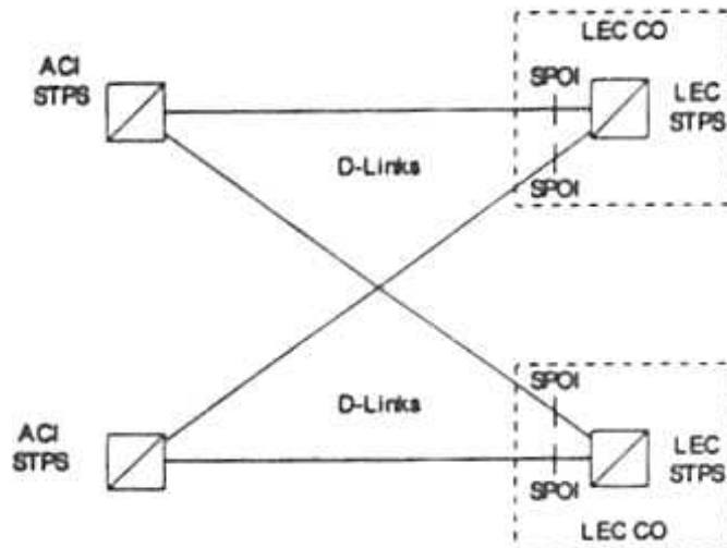
Figure 12. D-Link Interface
