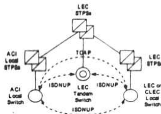
Figure 10. Inter-switch TCAP Signaling for SS7 Network Interconnection
