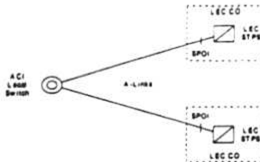
Figure 6. A-Link Interface
