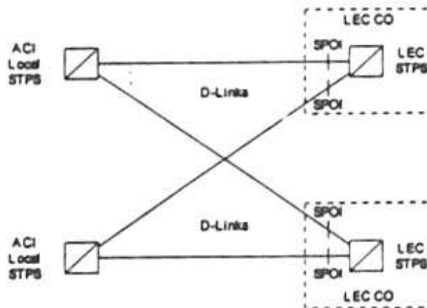
Figure 7. D-Link Interface
