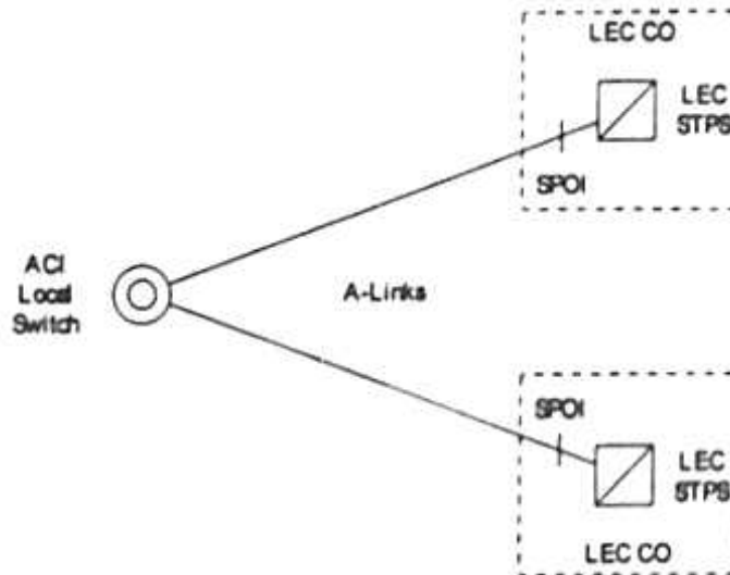
Figure 11. A-Link Interface
