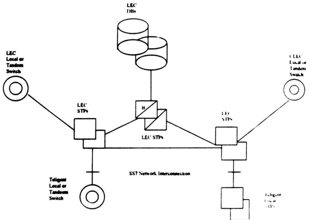
Figure 8. SS7 Network Interconnection
