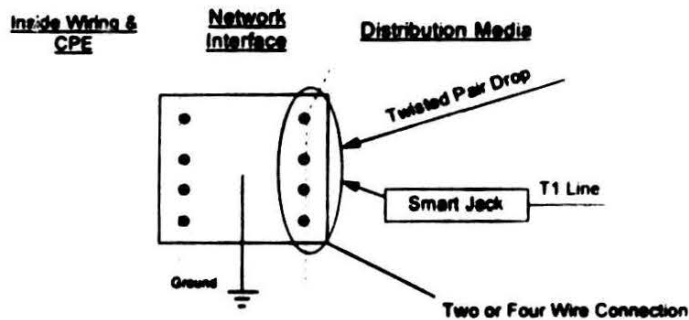
Figure 1 - Network Interface Device
