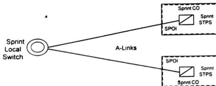
Figure 3. A-Link Interface
