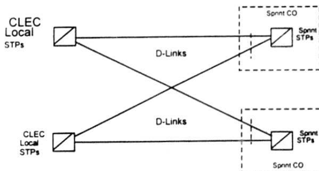
Figure 4. D-Link Interface
