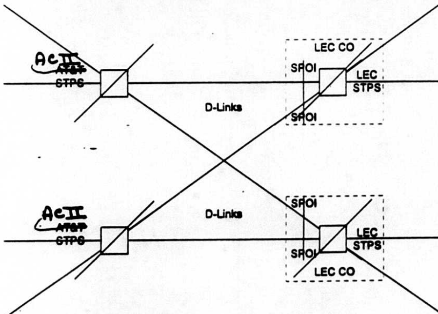
Figure 12. D-Link Interface
