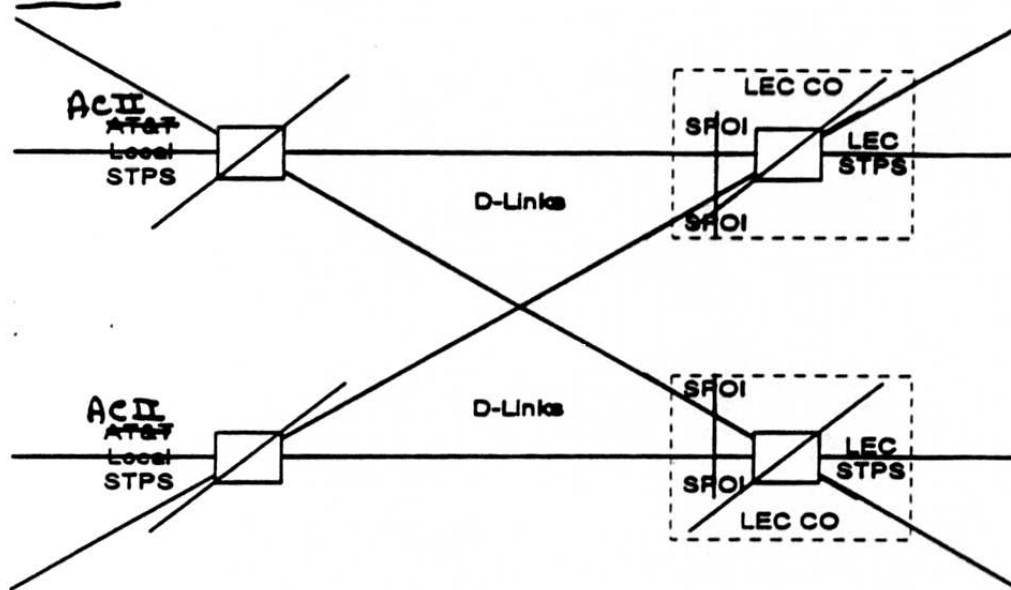
Figure 7. D-Link Interface
