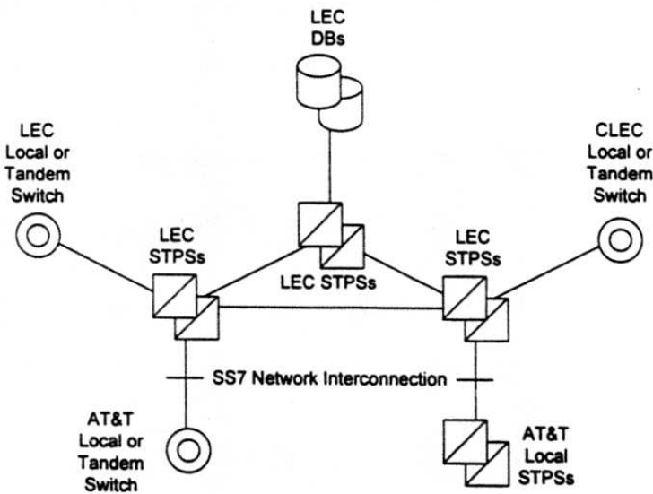
Figure 3. SS7 Network Interconnection
