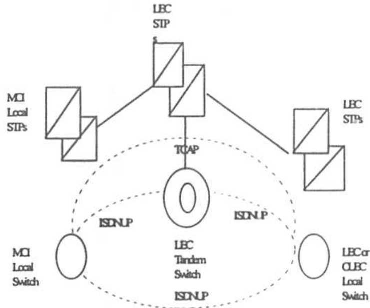
Figure 8. Interswitch TCAP Signaling for SS7 Network Interconnection
