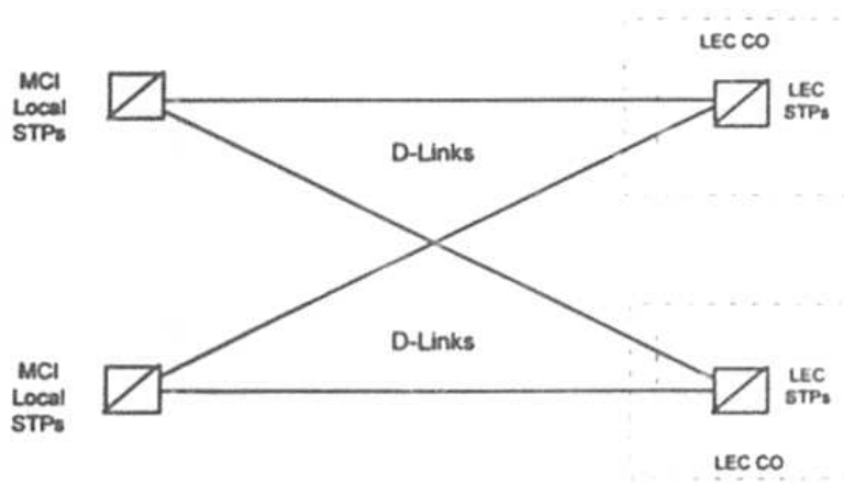
Figure 9. D-LINK Interface
