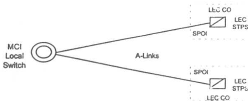
Figure 5. A-Link Interface
