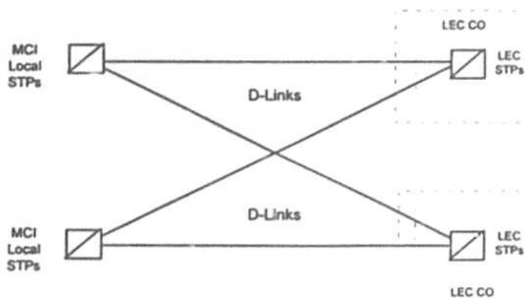
Figure 6. D-Link Interface
