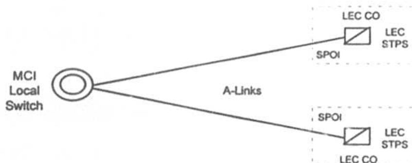
Figure 5. A-Link Interface
