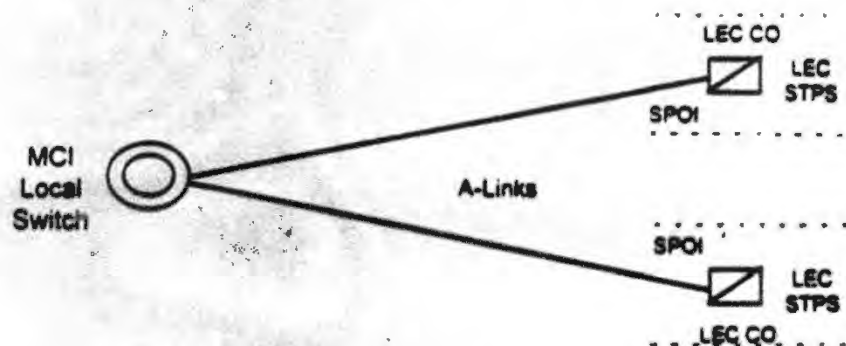
Figure 6. A-Link Interface
