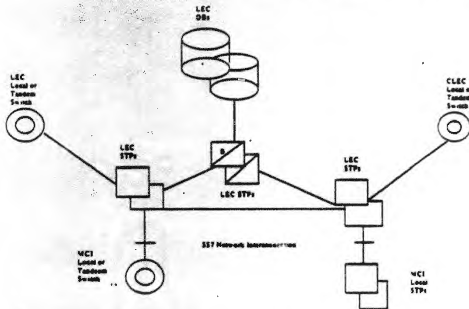
Figure 8. SS7 Network Interconnection
