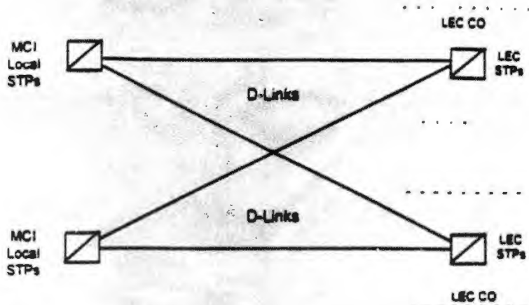
FIGURE 10. D-LINK Interface
