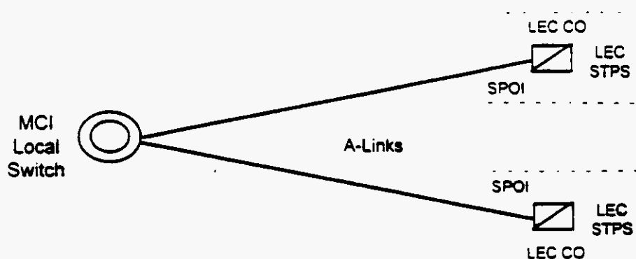
Figure 6. A-Link Interface
