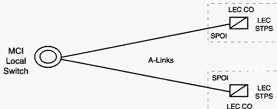
Figure 6. A-Link Interface
