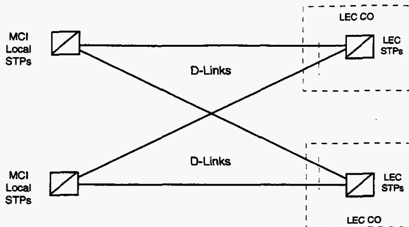
FIGURE 10. D-LINK Interface
