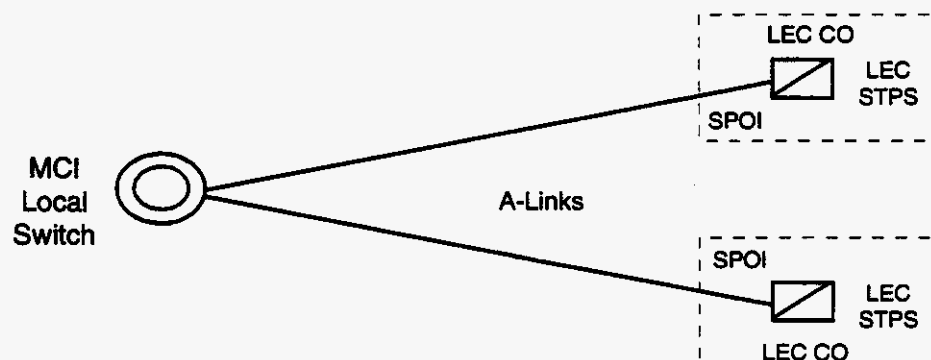
Figure 6. A-Link Interface
