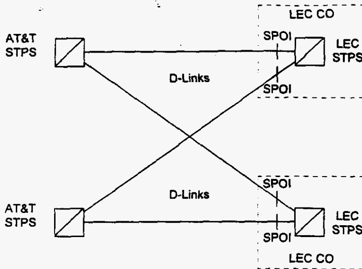
Figure 6. D-Link Interface
