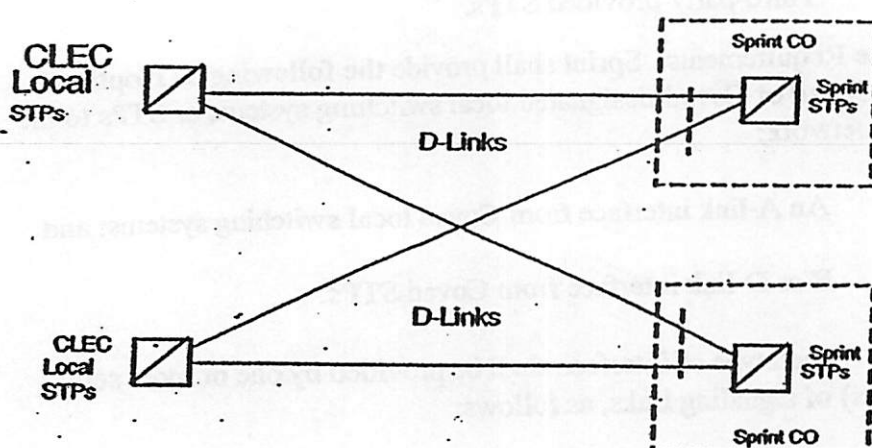
Figure 4. D-Link Interface
