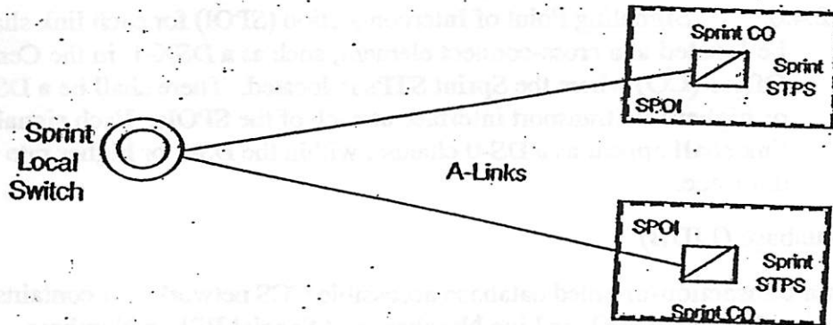
Figure 3. A-Link Interface
