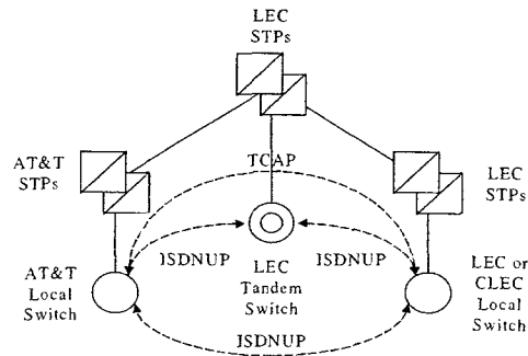
FIGURE 2 INTERSWITCH TCAP SIGNALING FOR SS7 NETWORK INTERCONNECTION
