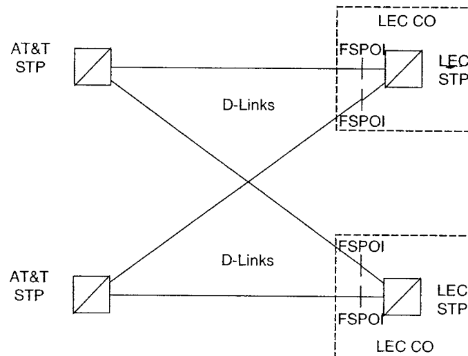
FIGURE 4. D-LINK INTERFACE
