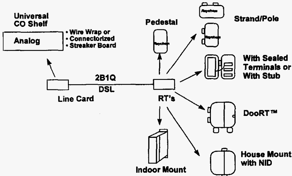
Figure 1: Raychem Miniplex 4N1 RT Packaging Options
