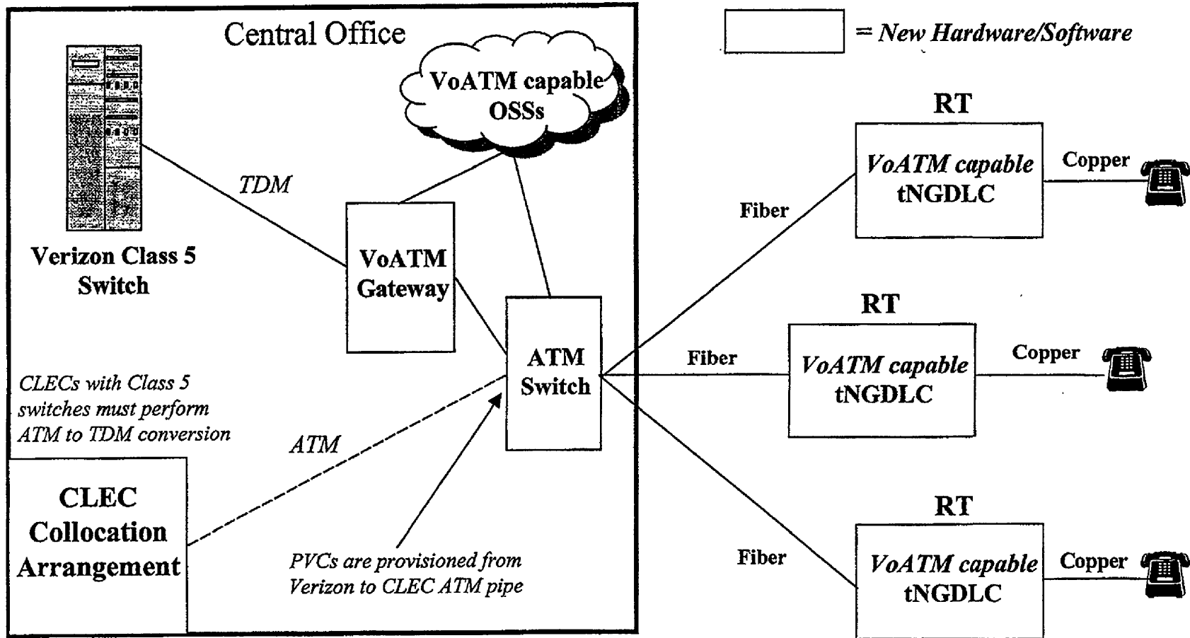
AT&T's Proposed Architecture for Electronic Loop Provisioning
