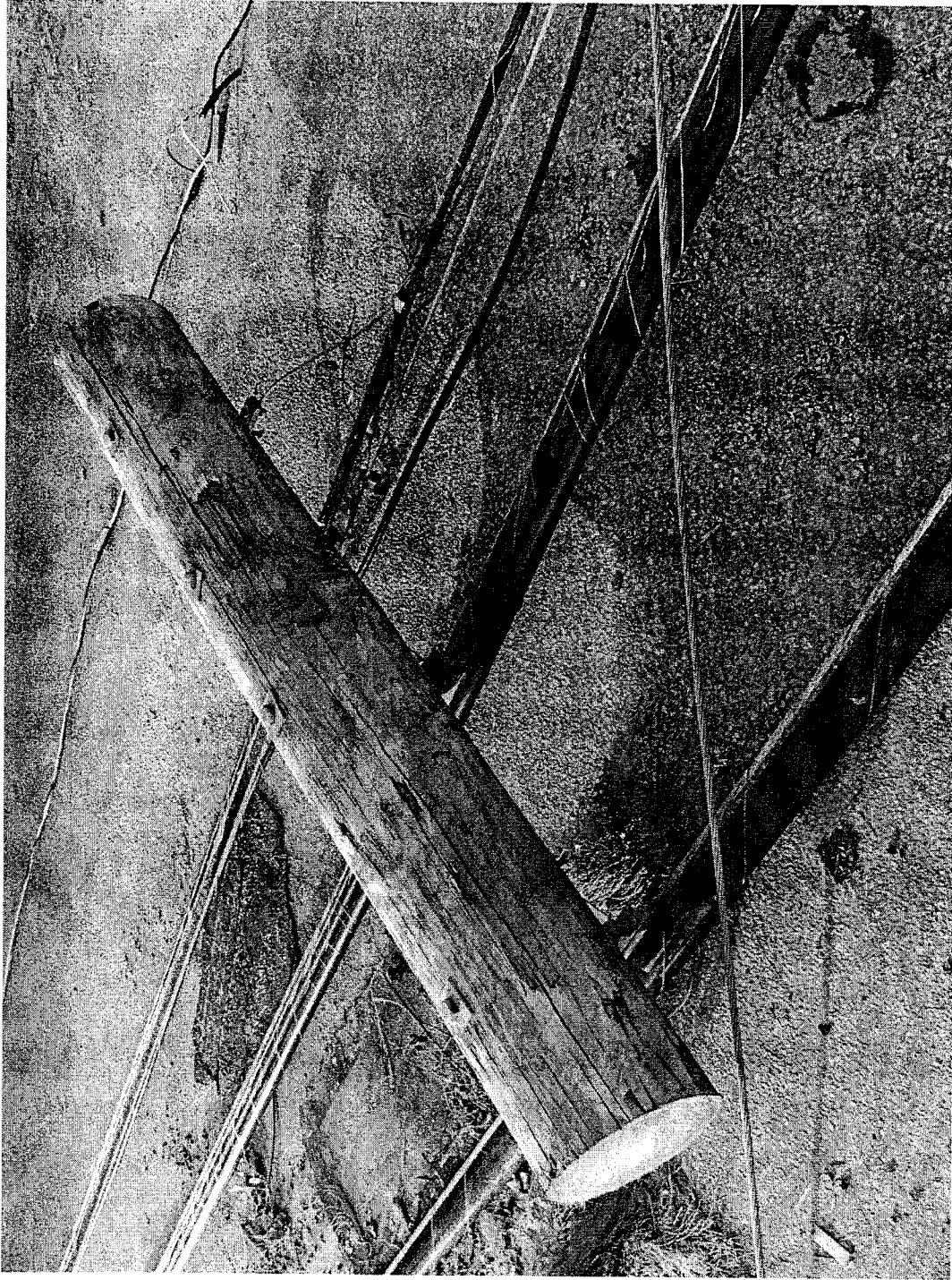
This healthy pole fell during the storm. It is burdened with a 2" telephone bundle, a 3" CATV bundle and a three cable telecommunication carrier bundle.
