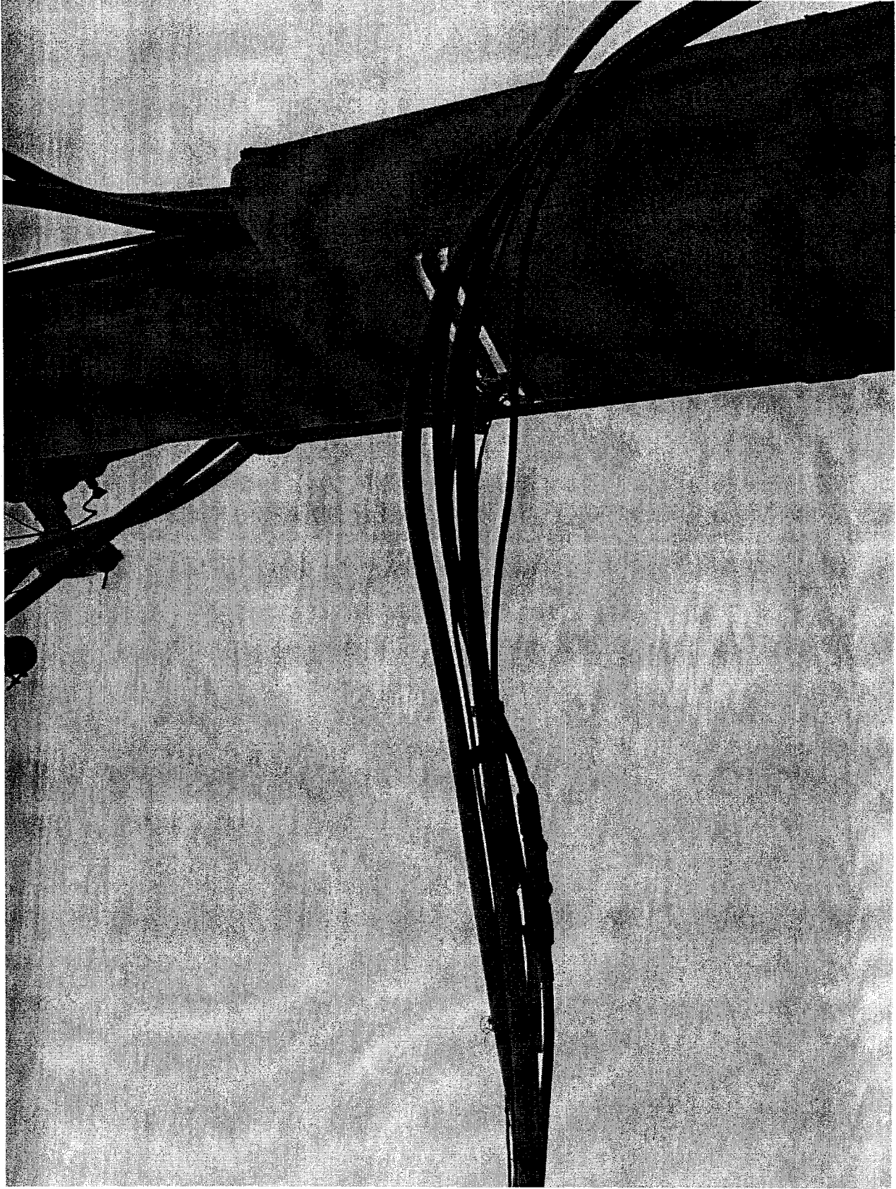
This bundle contains six cables and a messenger cable. Two of the cables are more than one inch in diameter. The bundle reaches a diameter of five inches and more where splices exist.
