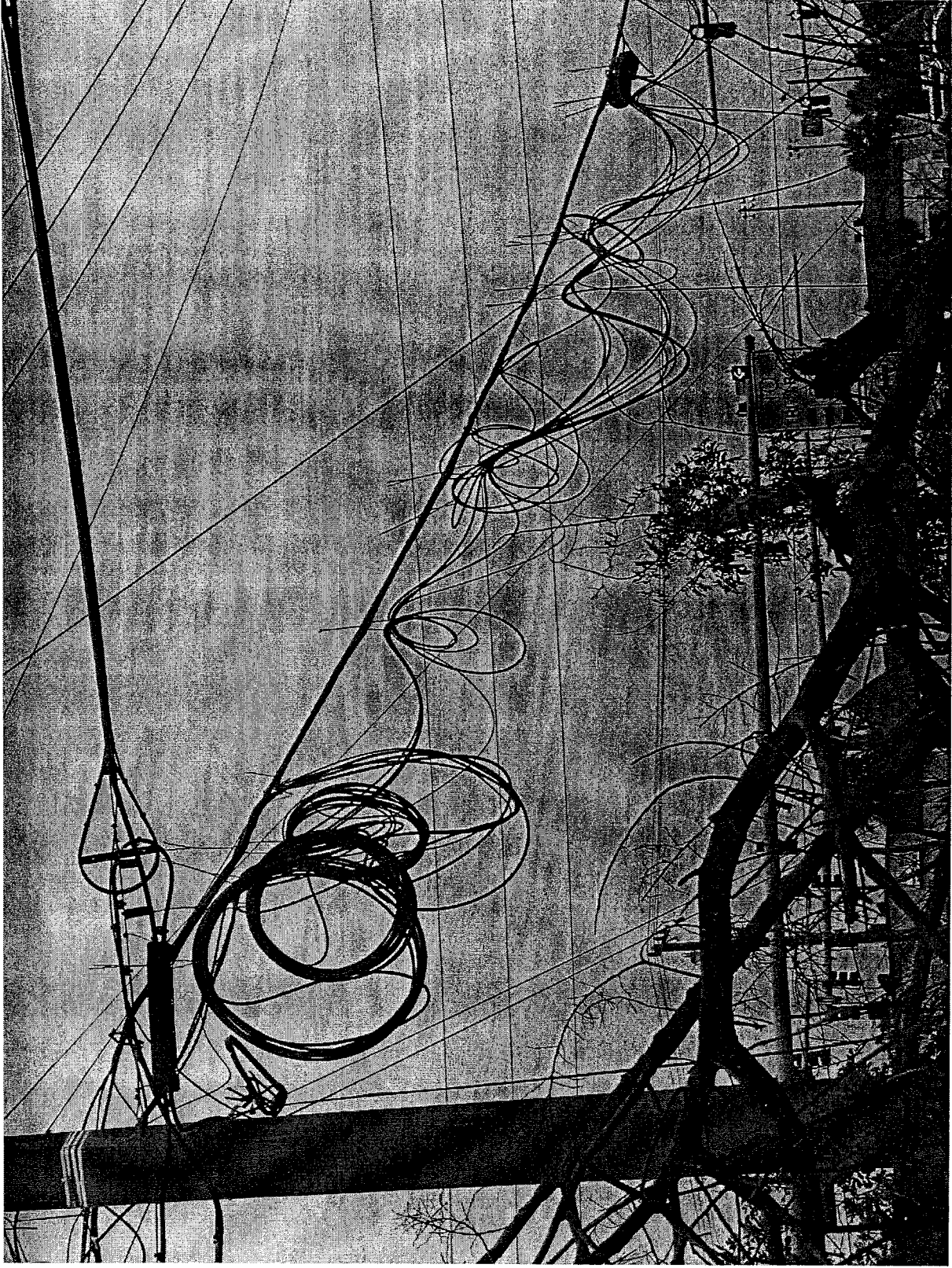
Very sloppily constructed CATV bundle with many cables attached along with a telephone bundle
