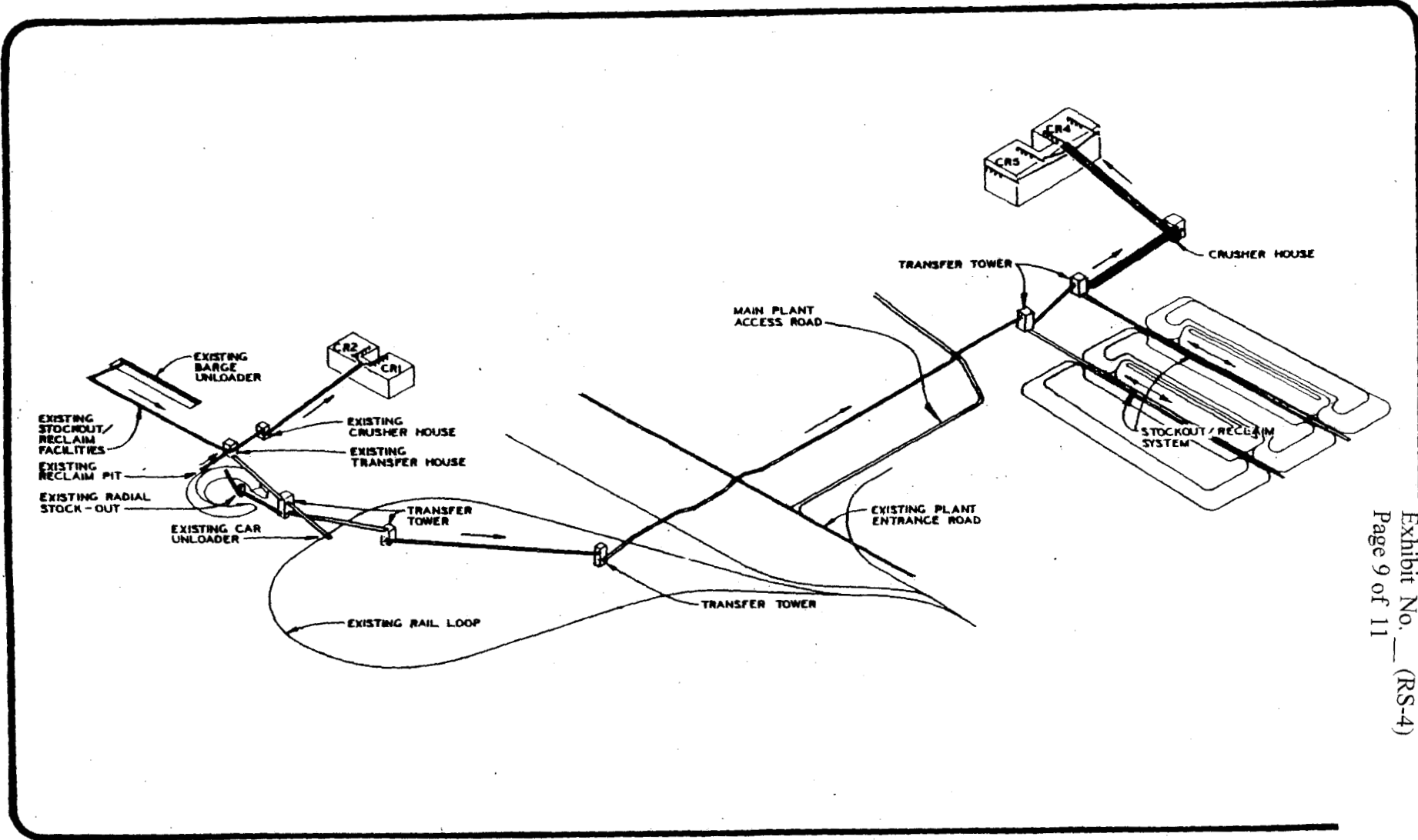
Figure 3.2-2 COAL HANDLING FACILITIES ISOMETRIC
