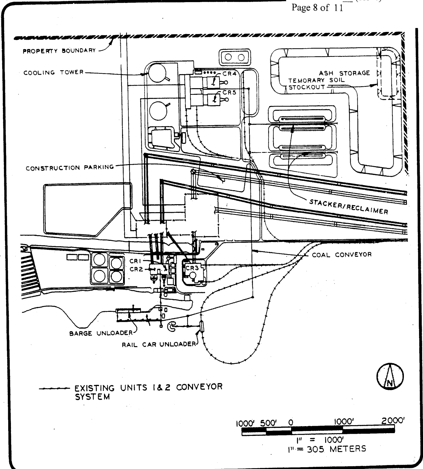
Figure 3.2-1 COAL HANDLING FACILITIES-CRYSTAL RIVER SITE SOURCE: BLACK AND VEATCH, 1980
