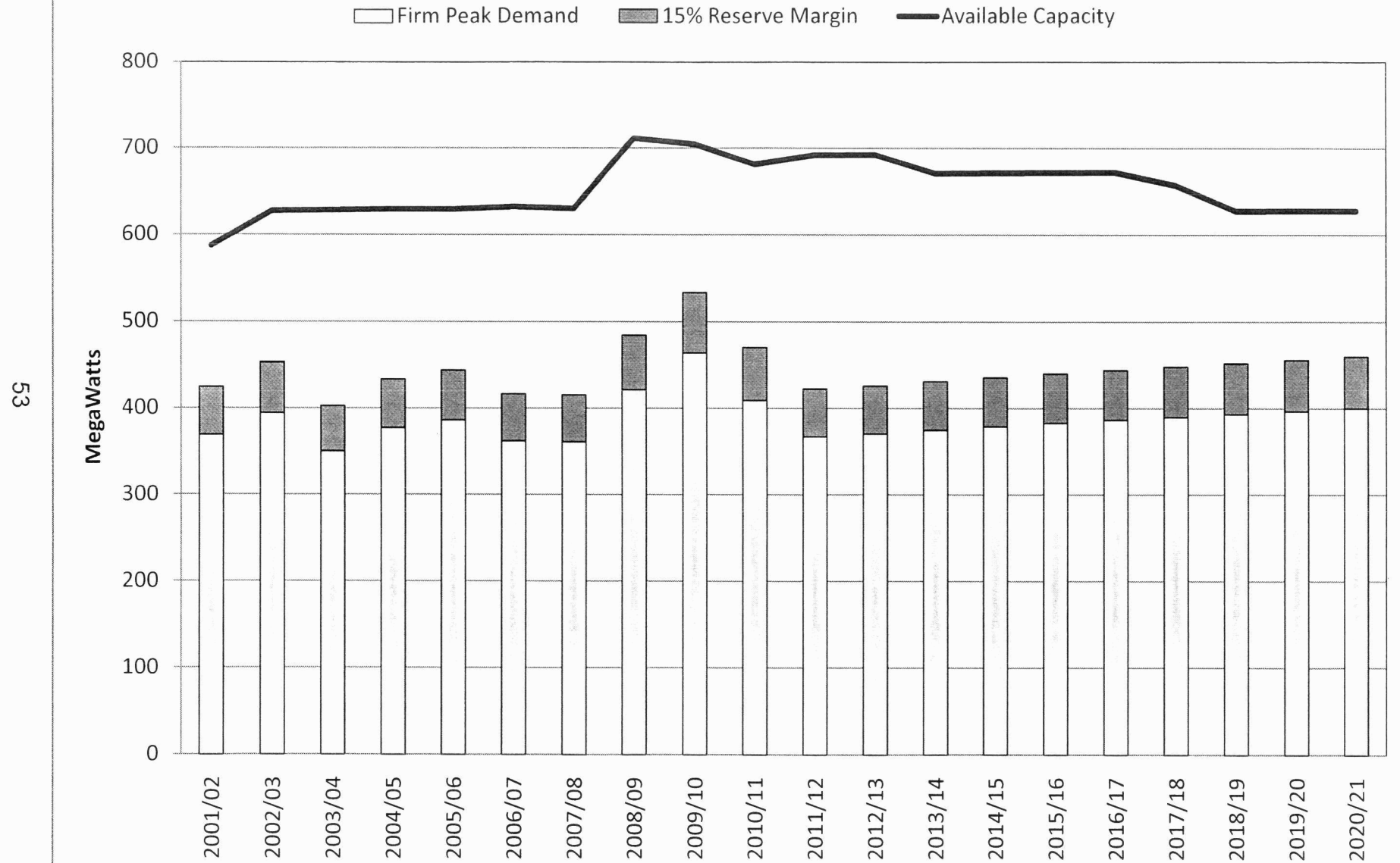
Figure 3.2 Winter Peak Demand and Resources
