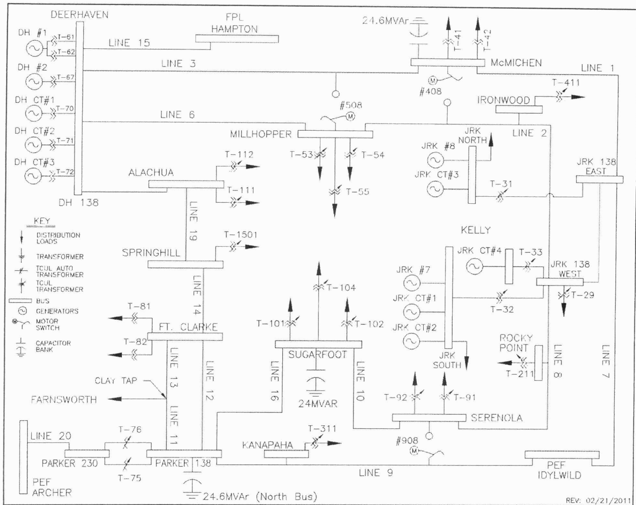
FIGURE 1.2 Gainesville Regional Utilities Electric System One-Line Diagram.
