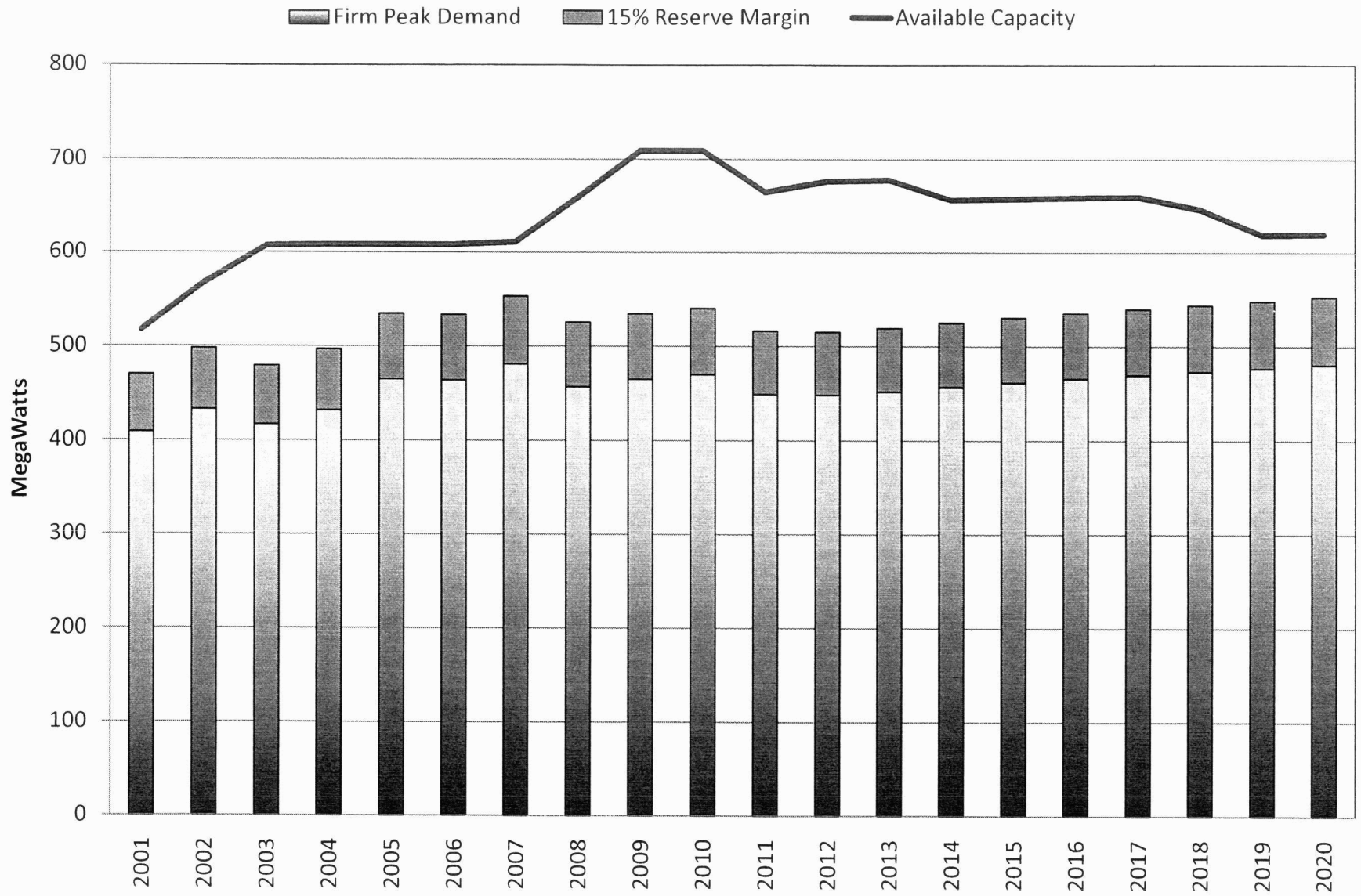
Figure 3.1 Summer Peak Demand and Resources
