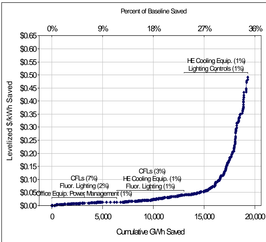
Figure 3-31: Commercial Energy Efficiency Supply Curve
