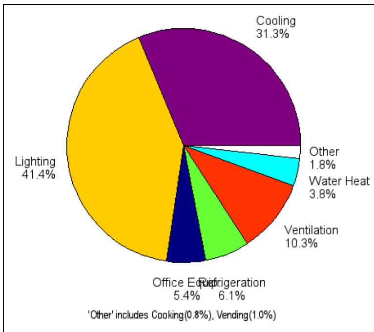
Figure 3-27: Estimated Breakdown of Total Technical Potential for Commercial Energy Savings in FPL by End Use (10,639 GWh)
