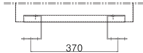
TOP VIEW Anchor DETAIL
