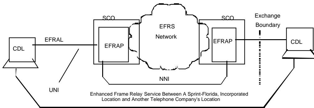
Sprint-Florida, Incorporated dba Sprint EFRS Diagram
