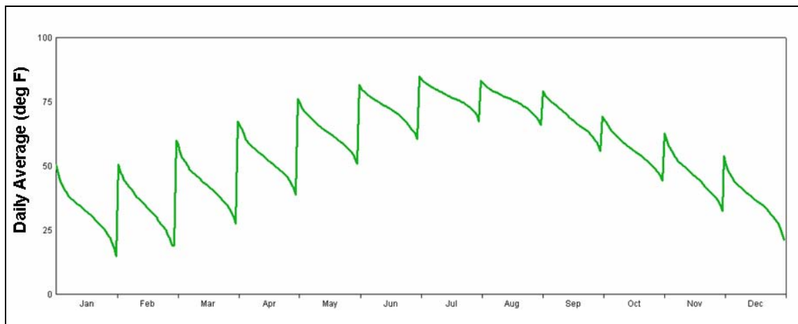
Figure 3: Example of Rank and Average Temperatures
