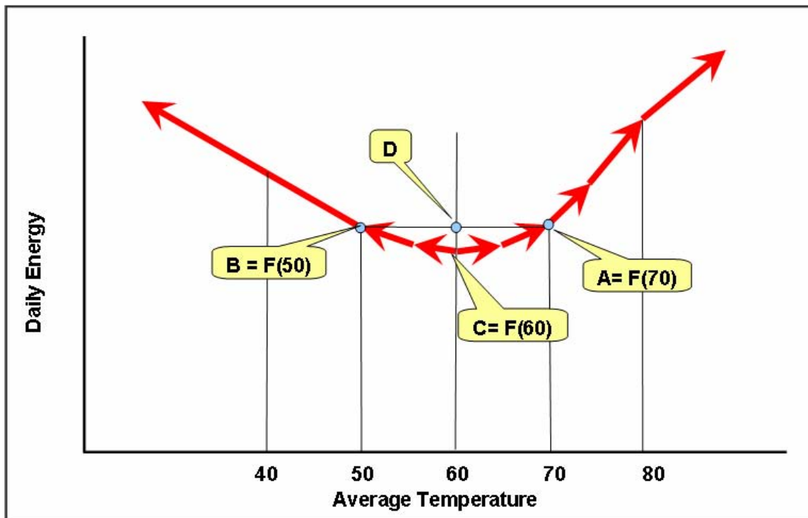
Figure 9: Example of Aggregation Bias – Averaging Across Years
