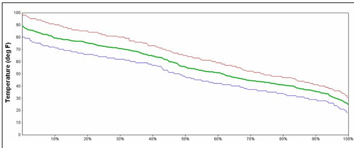
Figure 2: Example of one year of data ranked by average temperature
