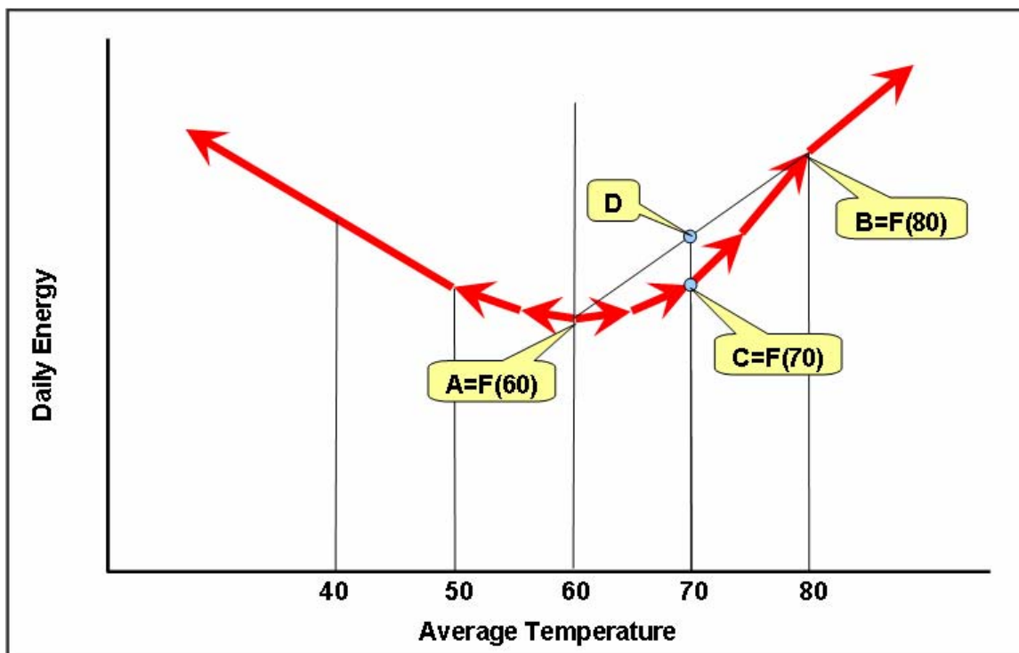
Figure 8: Example of Aggregation Bias – Averaging across Stations
