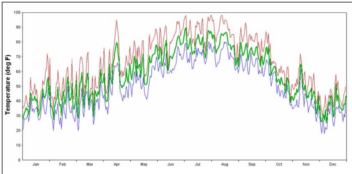
Figure 1: Example of actual weather data
