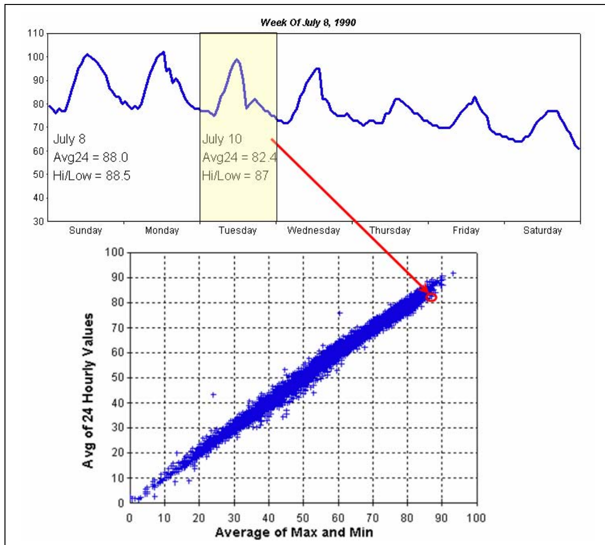
Figure 11: Example of High+Low/2 versus Average of Hourly Values
