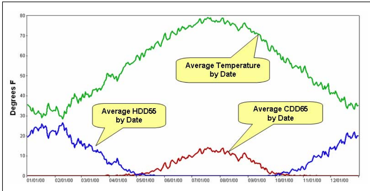
Figure 4: Example of Average by Data over 30 Years
