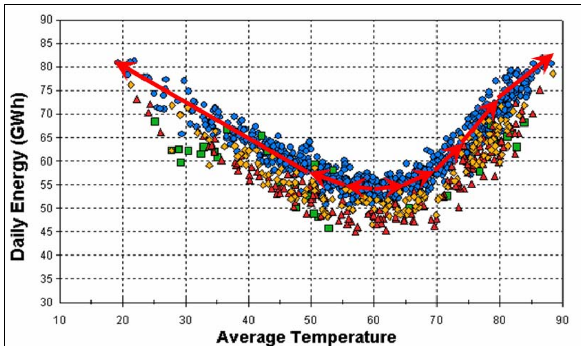
Figure 6: Example of Relationship between Energy and Temperature
