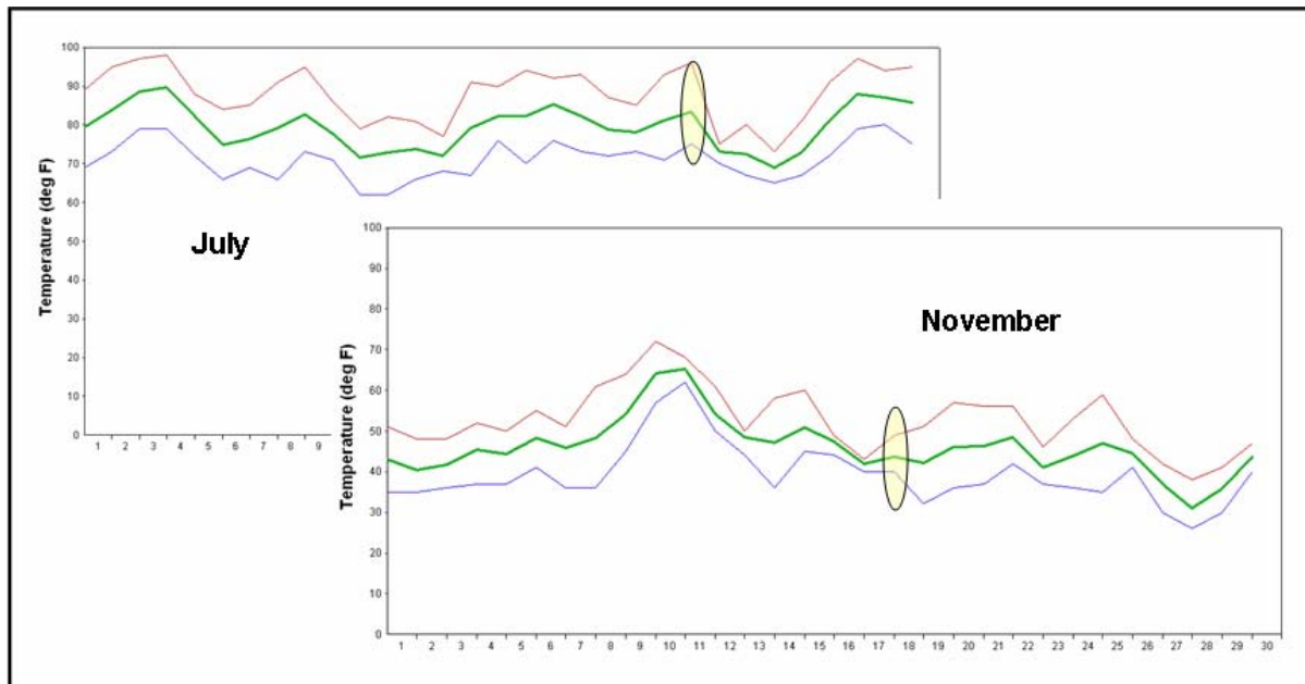
Figure 12: Examples of Peak Day Weather
