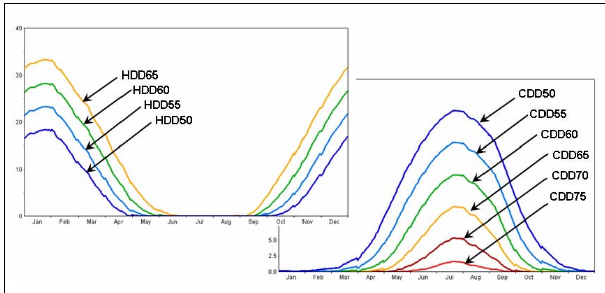
Figure 5: Example of CDD and HDD – Smoothed 30 Year Average by Date
