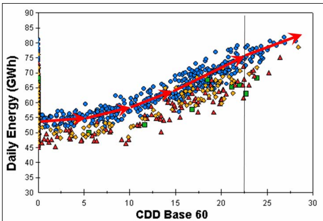
Figure 7: Example of Relationship between Energy and CDD60
