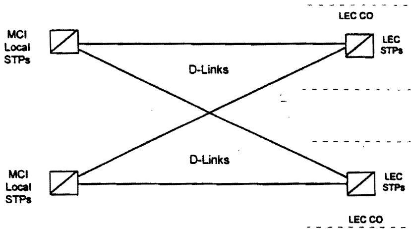
FIGURE 10. D-LINK Interface
