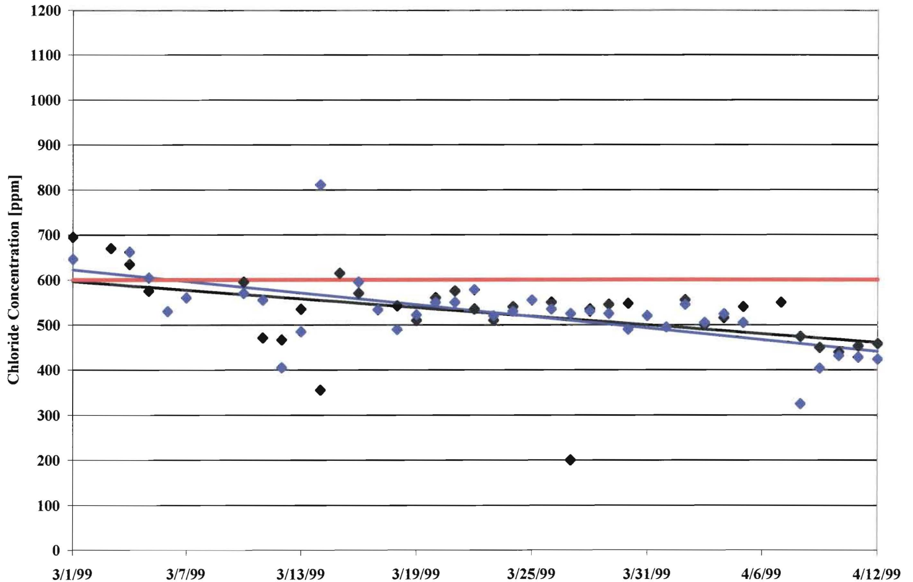
Figure 4. Effluent chloride concentrations from grab samples taken at 8 AM and 8 PM.
