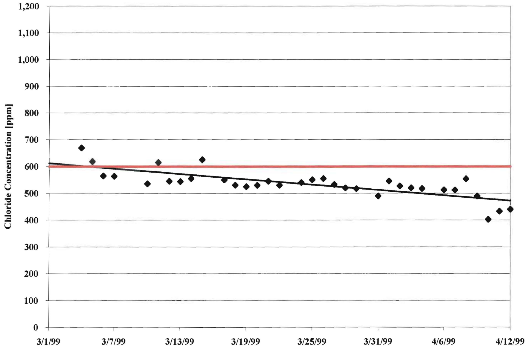
Figure 2. Composite chloride samples from effluent.
