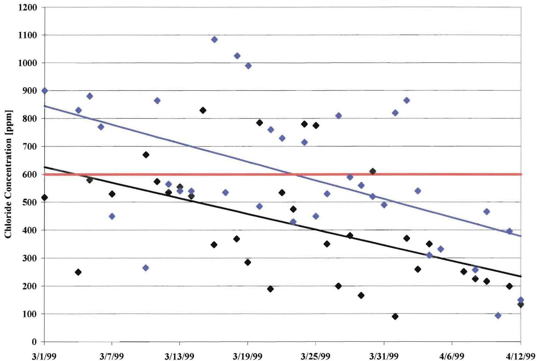
Figure 3. Influent chloride concentrations from grab samples taken at 8 AM and 8 PM.
