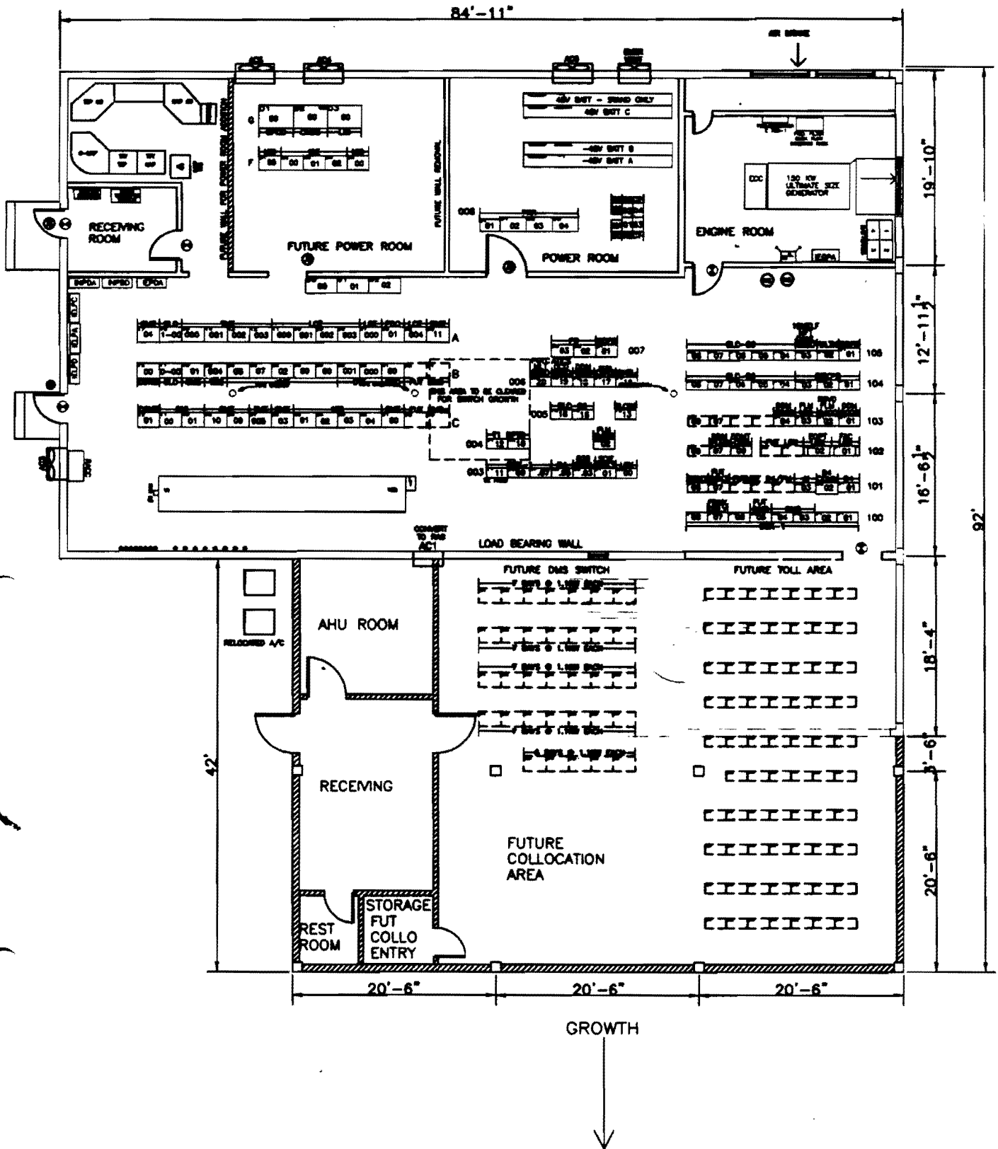
31488 HOLLY-NAVARRA FLOOR PLAN YEAR 2000 BUILDING ADDITION PSC WAIVER ITEM 4 G-H
