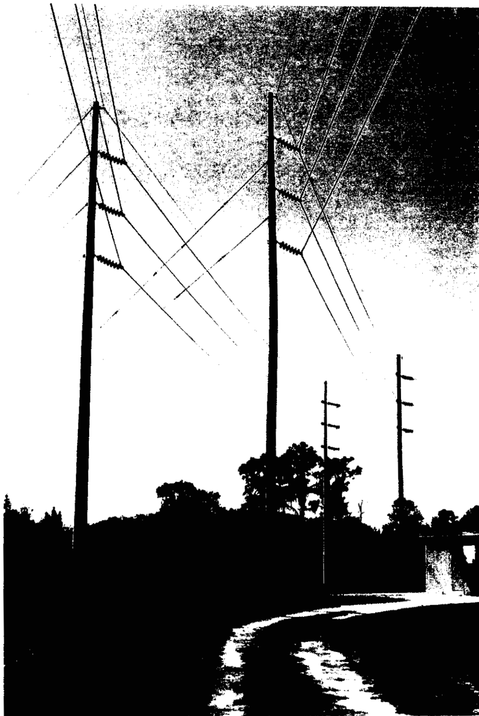
Picture 12: Typical single pole wood and concrete angle structures
