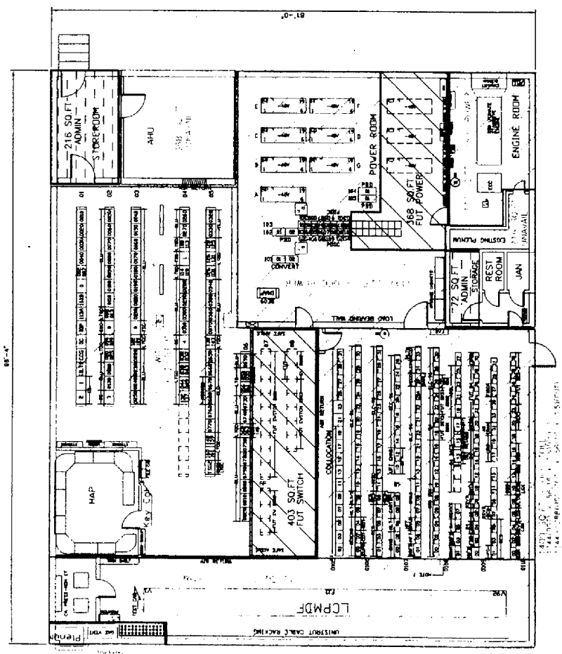
36010 MILTON RAVINE FLOOR PLAN PSC WAIVER ITEM 4 A-F PAGE 2
