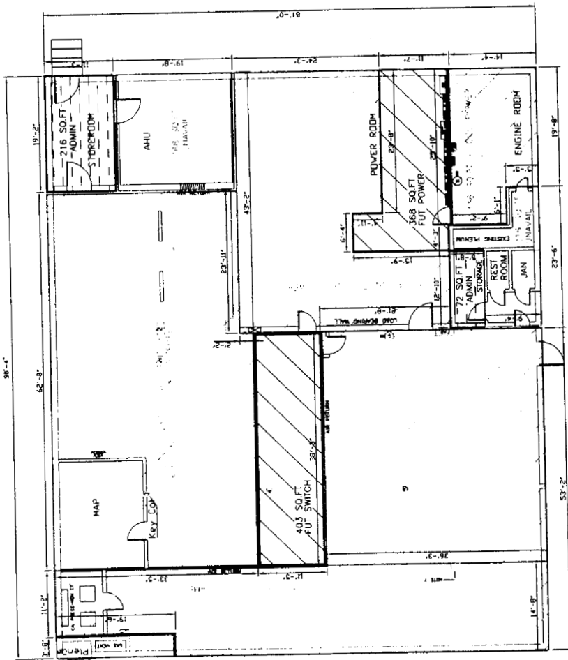
36010 MILTON RAVINE FLOOR PLAN PSC WAIVER ITEM 4 A-F PAGE 1
