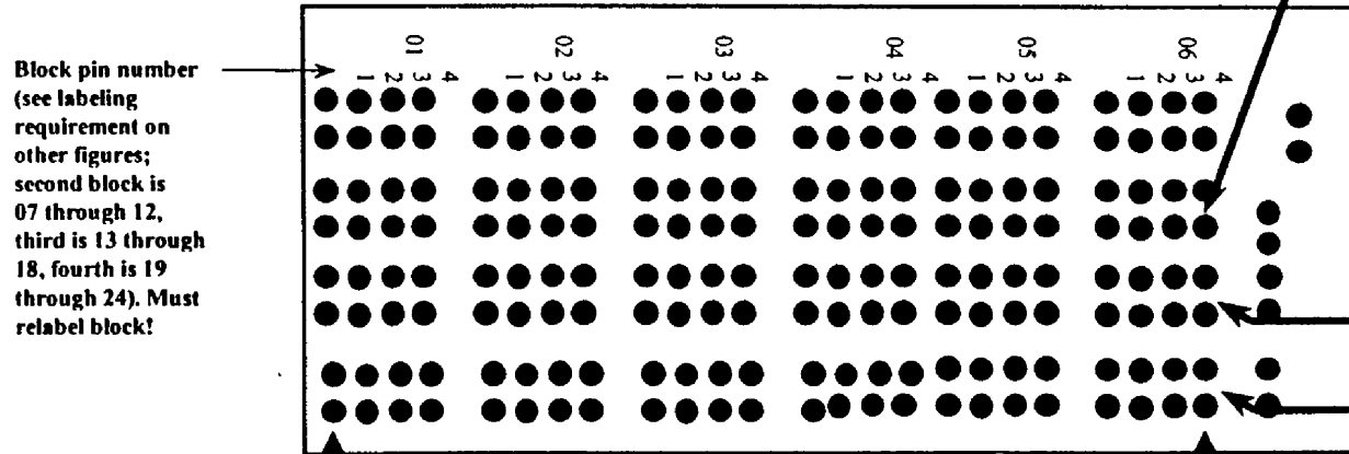
Figure 5 Wiring schematic Siecor 96 line splitter
