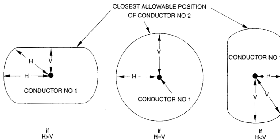
Figure 233-3—Clearance envelope
