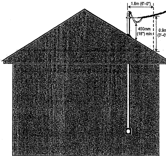
Elevation View
