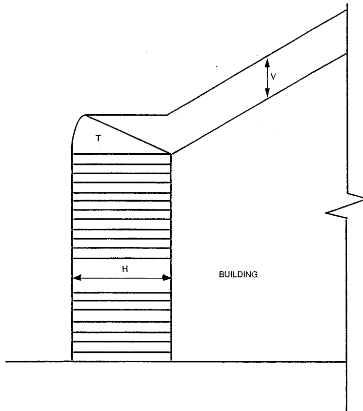
Figure 234-1(c)—Transitional clearance when H is greater than V
