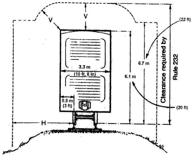
Figure 234-5—Rail car clearances
