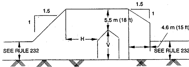
Figure 234-4(a)—Clearance envelope for grain bins filled by permanently installed augers, conveyors, or elevators
