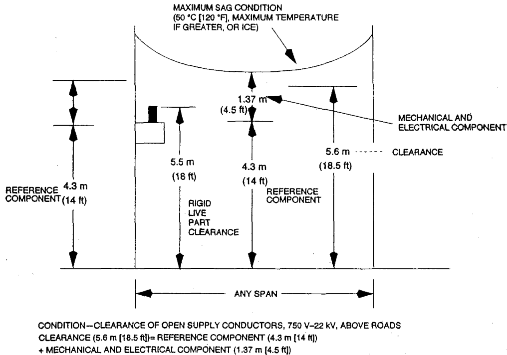
Figure A-1—Clearance at maximum sag
