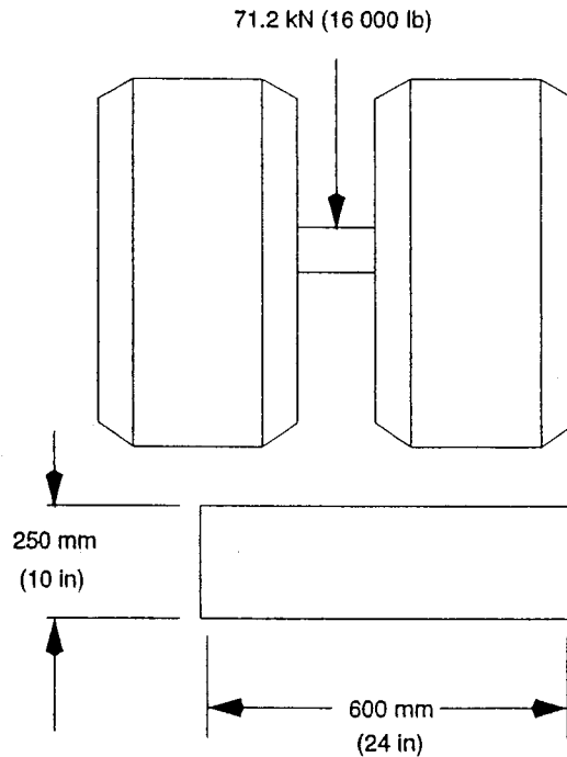
Figure 323-2—Wheel load area
