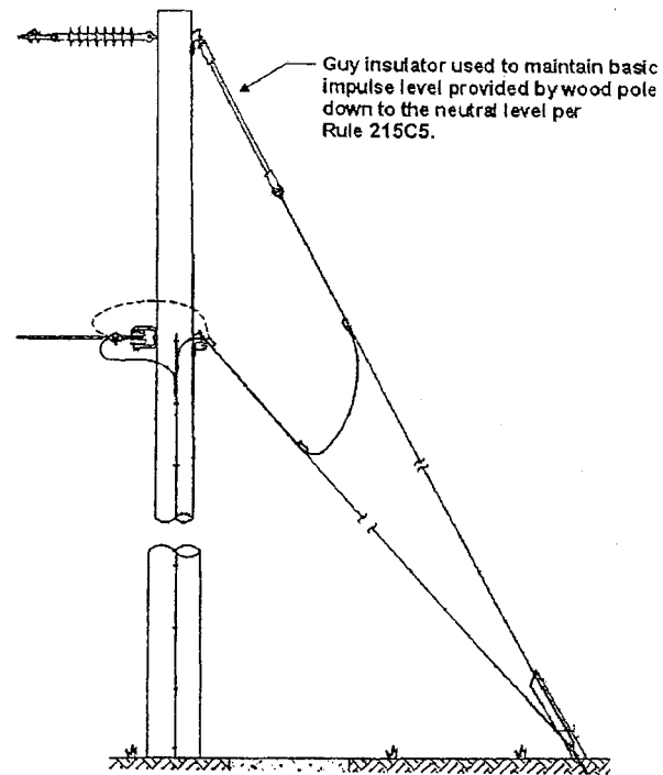
Figure 279-1—Insulator used for BIL insulation
