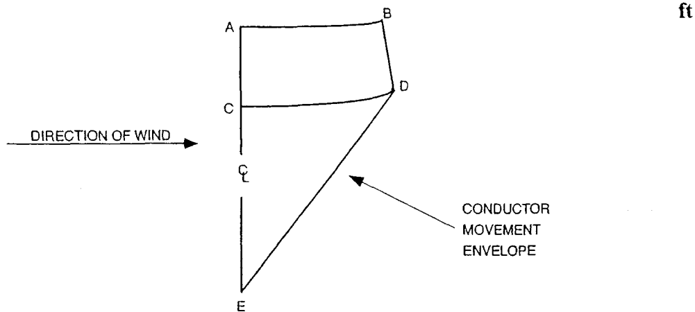
Figure 233-2—Conductor movement envelope
