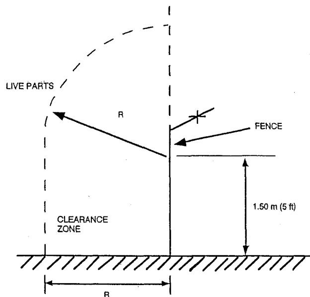
Figure 110-1—Safety clearance to electric supply station fences
