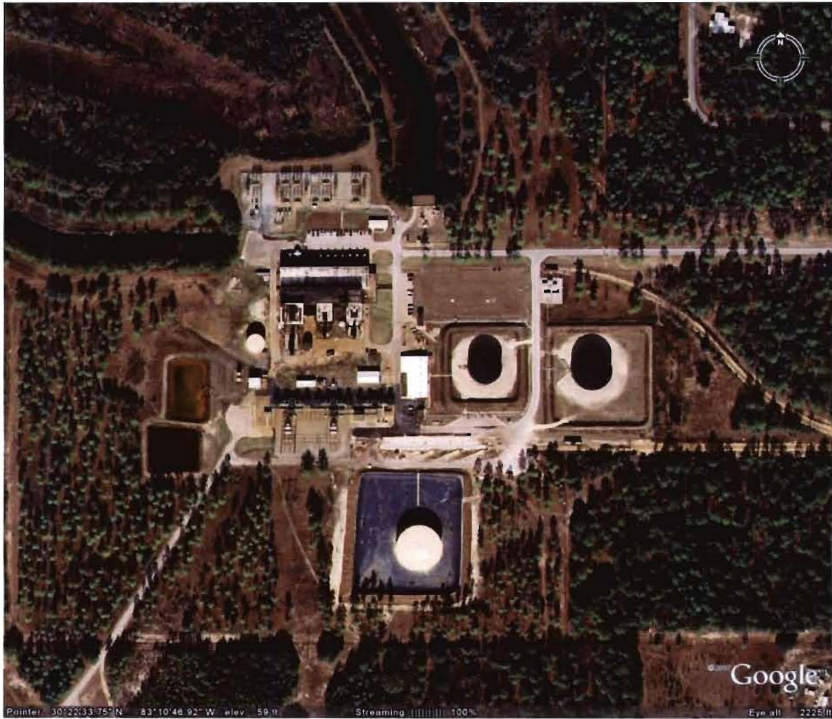
Suwannee River Plant (Suwannee County) –Plant Layout
