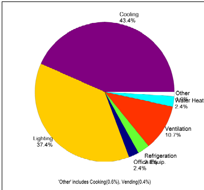
Figure 3-28: Estimated Breakdown of Total Technical Potential for Commercial Summer System Peak Demand Savings by End Use (4,079 MW)
