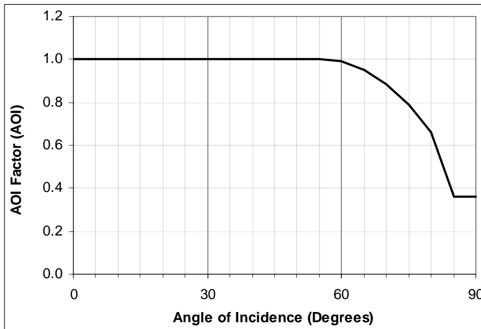
Figure 5-1: Angle of Incidence Factor
