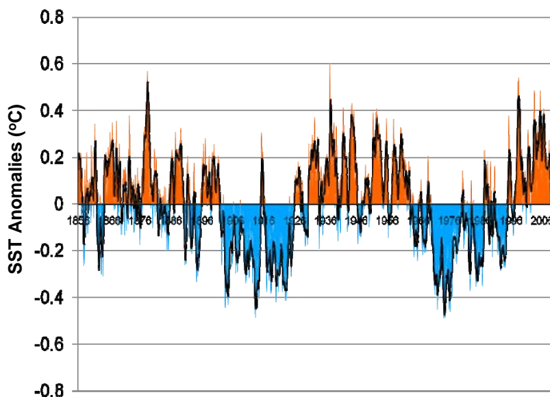
Figure 3-1: Atlantic Multidecadal Oscillation in Sea Surface Temperatures (SST) 1856-2010
