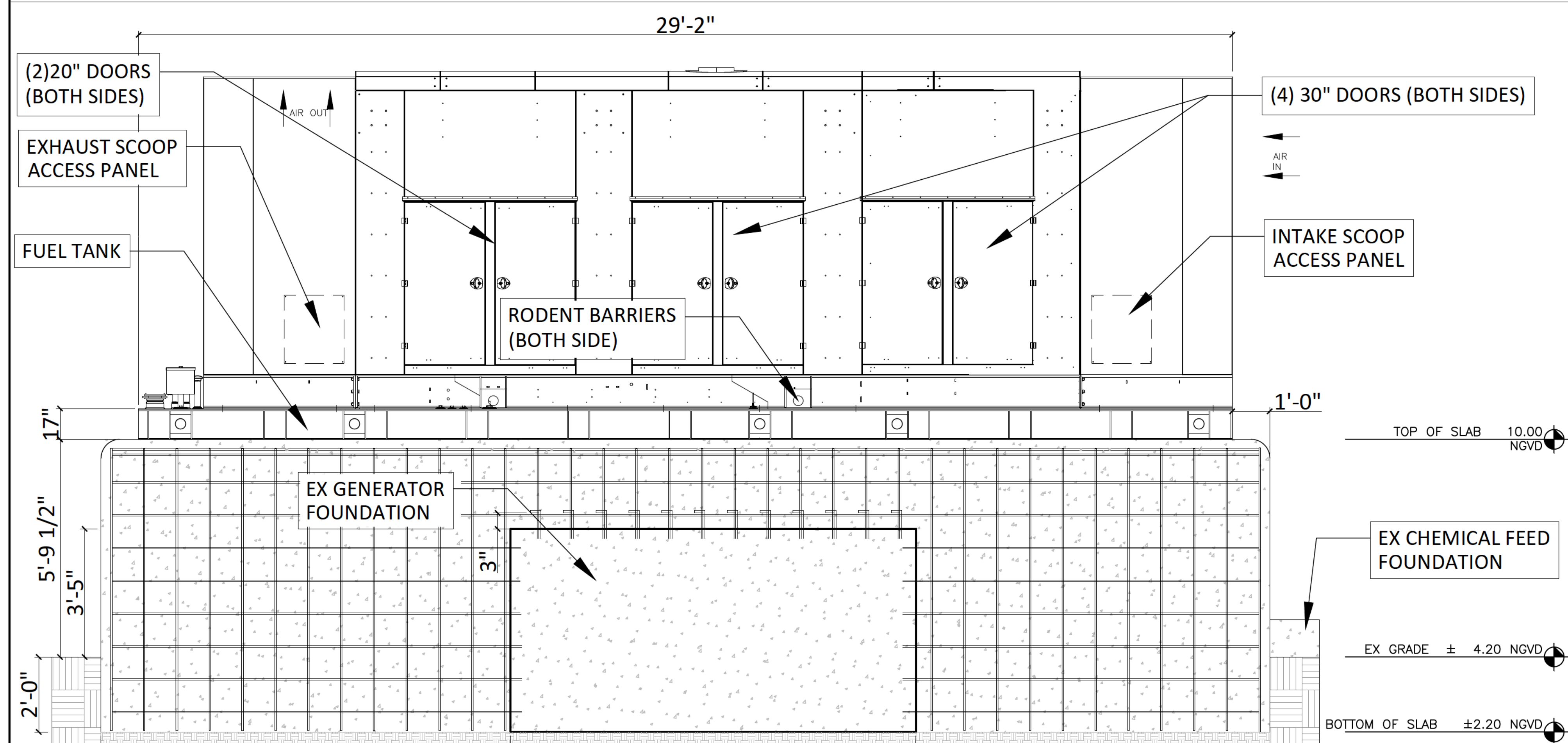
PROPOSED GENERATOR FOUNDATION DETAILS
